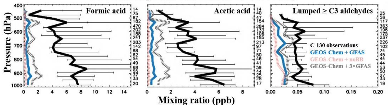
5 Figure S4. Median vertical profiles of VOC mixing ratios (formic acid, acetic acid, and lumped \geq C3 aldehydes) in the western US during the WE-CAN aircraft campaign (July-September 2018). GEOS-Chem simulation driven by GFAS is compared to observations. Also shown are two model sensitivity tests with biomass burning emission turned off (noBB) and with tripling GFASv1.2 emission ( 3 \times GFAS). Model results are sampled along the flight tracks at the time of flights; and observations are regridded to model resolution. Profiles are binned to the nearest 30 hPa. Horizontal bars show the 25 th -75 th percentile range of measurements in each vertical bin. The number of observations in each bin is given on the right side of each panel.
