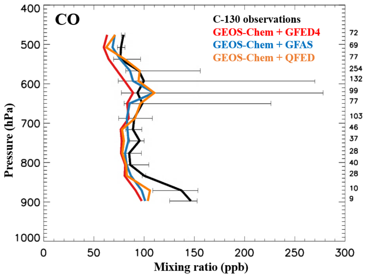
Figure S5. Median vertical profiles of CO mixing ratios in the western US for low/no smoke conditions in the WE-CAN aircraft campaign. GEOS-Chem simulations driven by three different biomass burning emission inventories (GFED4s, GFASv1.2, and QFED2.4) are compared to observations. Results are filtered to include only data coincident with the bottom 25th percentile of observed acetonitrile, where EnRs of CH 3 CN to CO larger than 2.01 ppb ppm -1 , and where the number of datapoints are larger than 5. Model results are also sampled along the flight tracks at the time of flights; and observations are regridded to model resolution. Profiles are binned to the nearest 30 hPa. Horizontal bars show the 25 th -75 th percentile range of measurements in each vertical bin. The number of observations in each bin is given on the right side of each panel.
