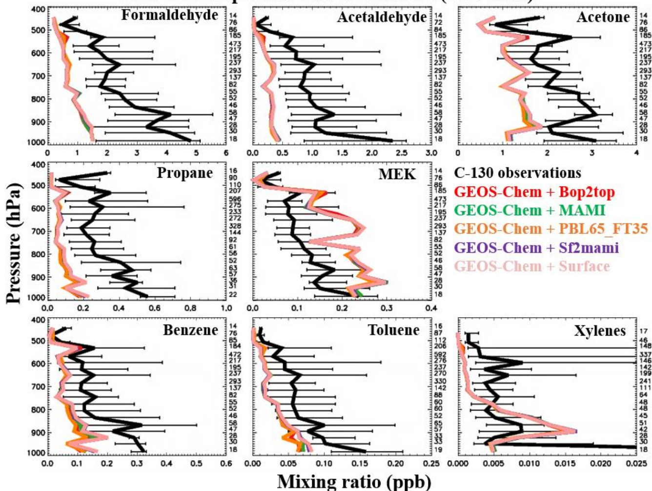
20 Figure S6. The median vertical concentration profiles of 8 VOCs observed during WE-CAN (black, solid) over the western US. Also shown are GEOS-Chem simulations driven by GFASv1.2 in five injection schemes: 1) releasing BB emissions evenly from bottom of the plume to the top of the plume (Bop2top, red); 2) emitting BB at the mean altitude of maximum injection (MAMI, green); 3) emitting 65% of BB emissions into planetary boundary layer and 35% into free troposphere (PBL65FT35, orange); 4) emitting BB evenly from the surface to the mean altitude of maximum injection (Sf2mami, purple); 5) emitting BB at surface (Surface, pink).
