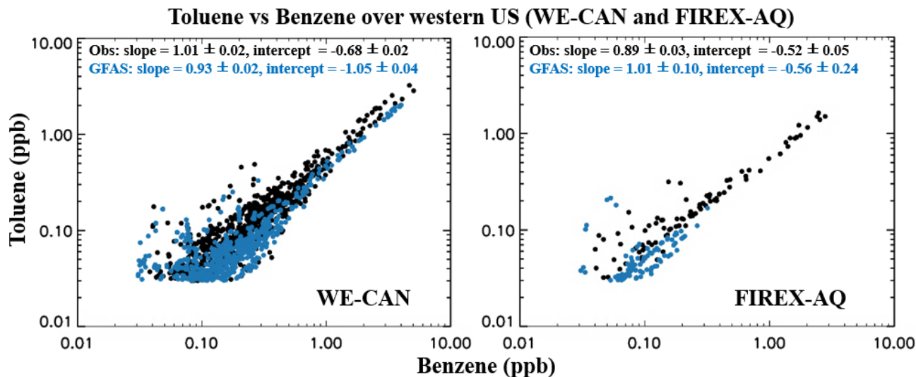
Figure S8. Relationship between benzene and toluene in the western US during WE-CAN (left) and FIREX-AQ (right). Data are plotted on a log-log scale, with observations in black and corresponding GEOS-Chem + GFAS simulations in blue. Model results are sampled along the flight tracks at the time of flights; and both the observations and the model outputs are regridded to model resolution (5 min and 0.25^\circ \times 0.3125^\circ ). The regression parameters shown represent the best fit of the data using the reduced major axis regression, corresponding to the relationship between \log_{10}(\text{benzene}) and \log_{10}(\text{toluene}) .
