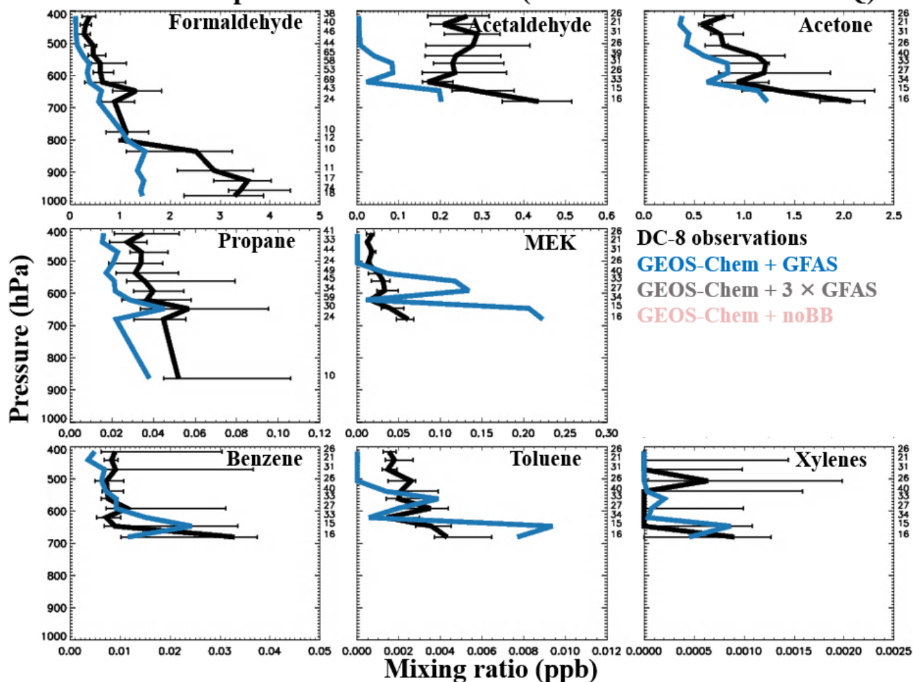
Figure S10. Median vertical profiles of observed VOC mixing ratios in the western US for low/no smoke conditions sampled in FIREX-AQ. Observations are compared to GEOS-Chem simulation driven by GFASv1.2. Results are filtered to include only data coincident with the bottom 25 th percentile of observed acetonitrile, where \Delta\text{CH}_3\text{CN}/\Delta\text{CO} larger than 2.01 ppb ppm -1 , and where the number of datapoints of each pressure bin are larger than 5. Model results are also sampled along the flight tracks at the time of flights; and both observations and model outputs are regridded to model resolution. Profiles are binned to the nearest 30 hPa. Horizontal bars show the 25th-75th percentile range of measurements in each vertical bin. The number of observations in each bin is given on the right side of each panel.
