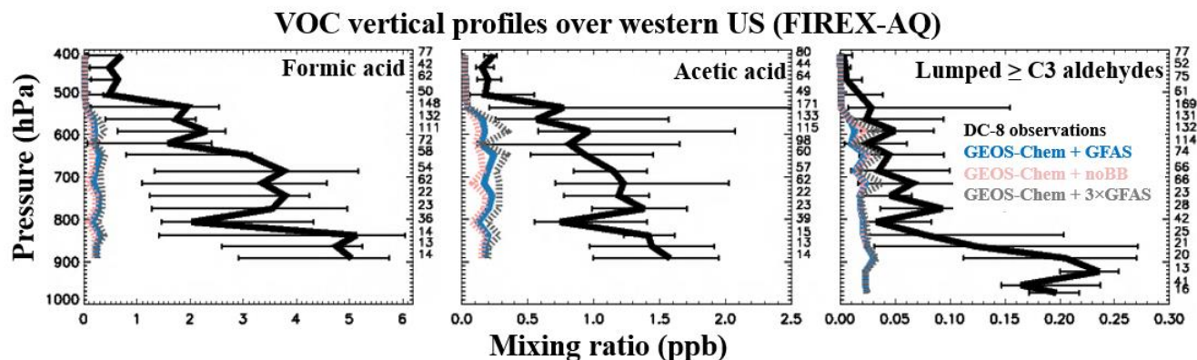
Figure S9. Median vertical profiles of three observed VOC mixing ratios in the western US during the FIREX-AQ aircraft campaign (July-September 2019). GEOS-Chem driven by GFASv1.2 is compared to observations. Also shown are two model sensitivity tests with biomass burning emission turned off (noBB) and with tripling GFASv1.2 emission ( 3 \times GFAS). Model results are sampled along the flight tracks at the time of flights; and both the observations and model outputs are regridded to the model resolution. Profiles are binned to the nearest 30 hPa. Horizontal bars show the 25 th -75 th percentile range of measurements in each vertical bin. The number of observations in each bin is given on the right side of each panel. Results are filtered to include only data where the number of datapoints for the pressure bin is larger than 10.
