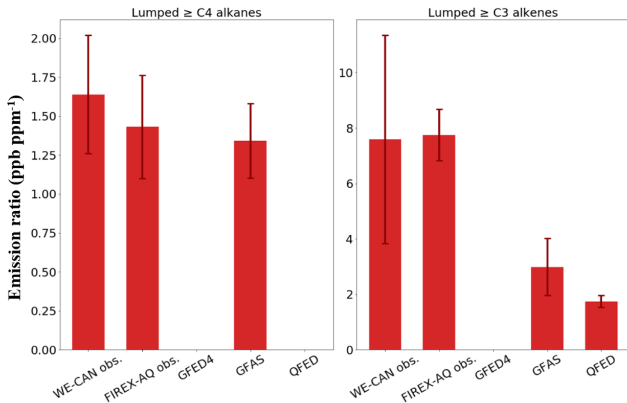
Figure S7. Biomass burning VOC emission ratios for western US wildfires observed on the C-130 during WE-CAN and the DC-8 during FIREX-AQ. Also shown are the emission ratios in GEOS-Chem simulations driven by three different BB emission inventories. Values of zero indicate that the species were not included in the BB emission inventory in the standard GEOS-Chem. Emission ratios are calculated from the reduced major axis regression (RMA) of VOC and CO, with error bars representing the 95% confidence interval from the bootstrapping resampling of the regression. R > 0.7 is used as the threshold in the RMA regression for ER calculations.
